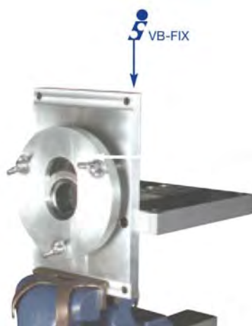
Universal Valve Body Reaming Fixture By Sonnax®
